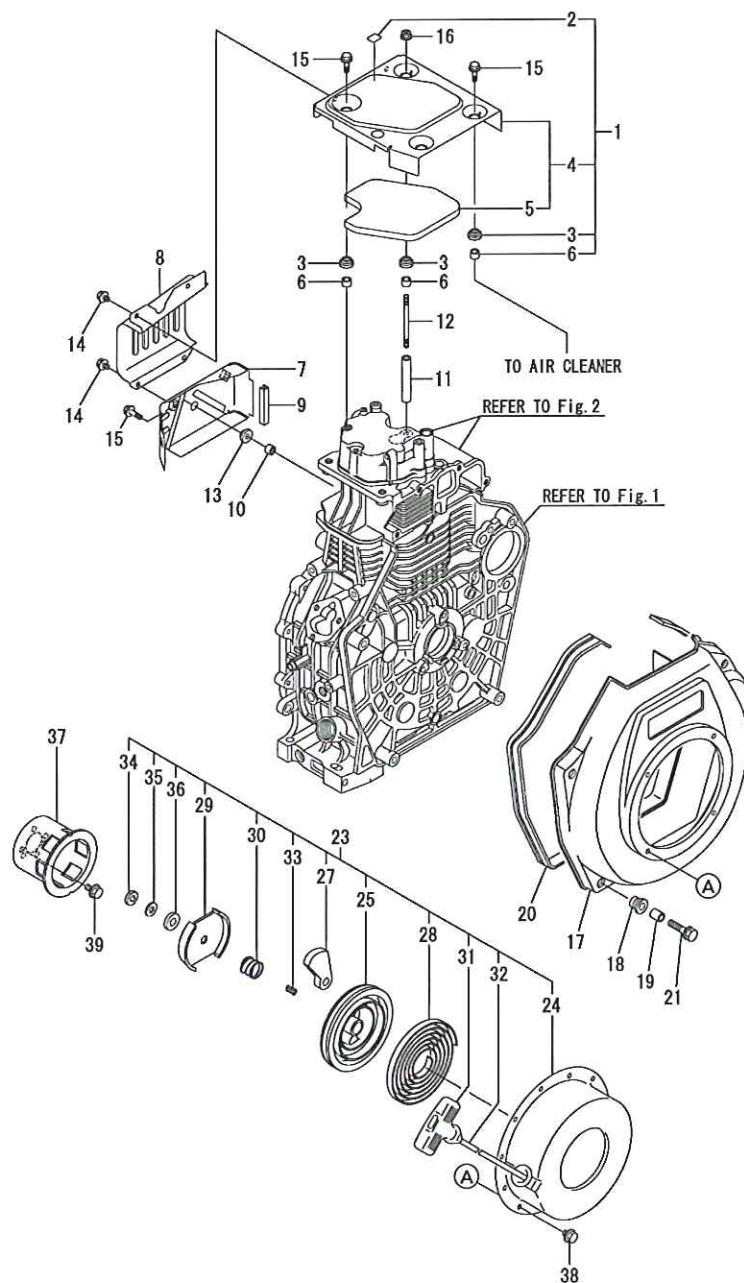
Fig.6. COOLING &amp; STARTING DEVICE
